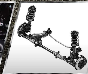
MacPherson Strut with stabilizer front suspension
